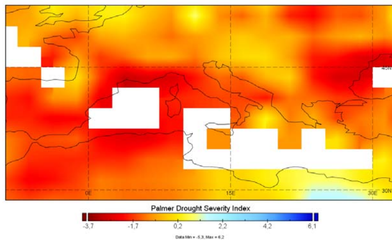
Monthly self-calibrated Palmer Drought Severity Index (Giugno 2009)
